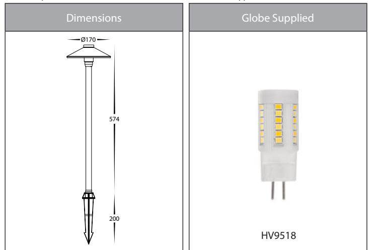
HV1452T-AB Antique Brass HV1452T-BLK SS316 Black HV1452T-CP Solid Copper HV1452T-SS316 SS316
