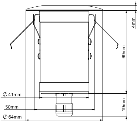
Core Hole Cutout: 50 ~ 55mm
